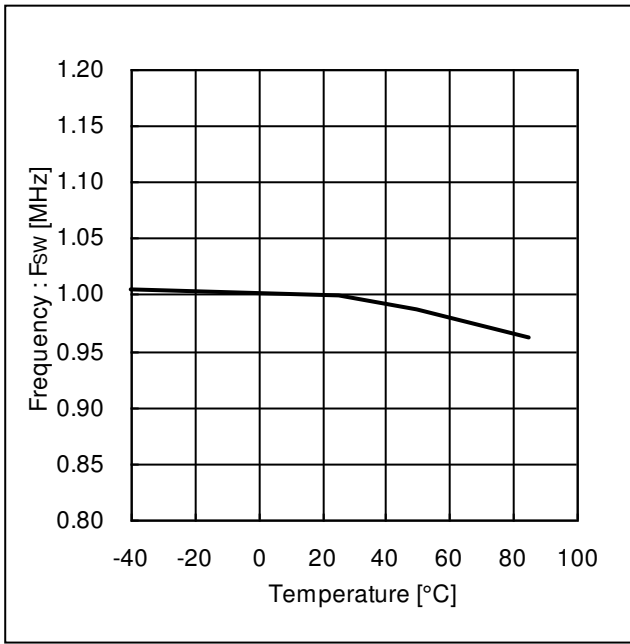
Figure 5. Oscillator Frequency - Temperature
