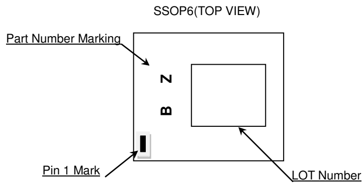
Figure 48. Marking Diagram
