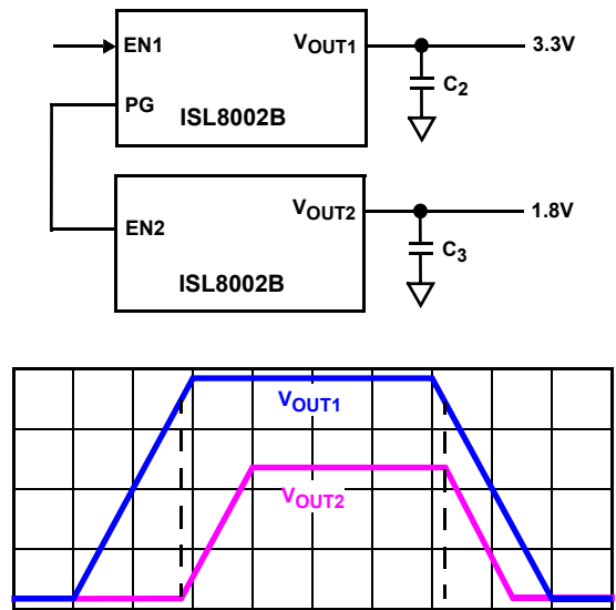
FIGURE 61. OUTPUT SEQUENCING
