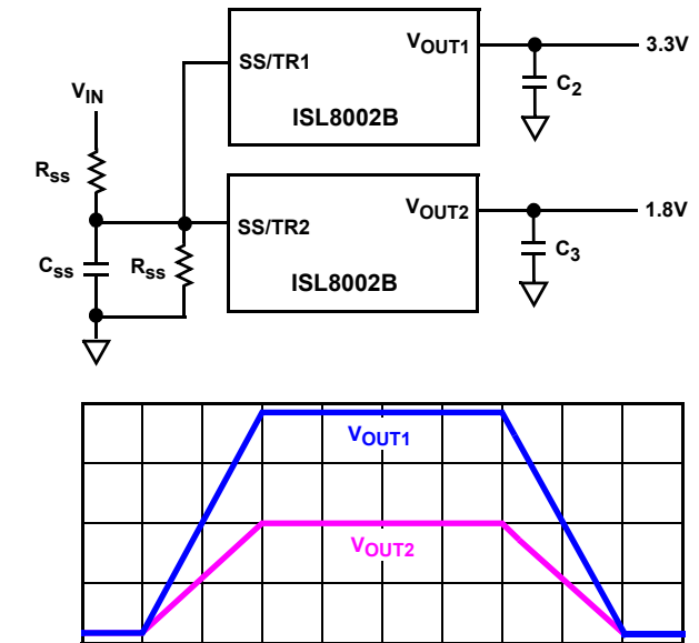
FIGURE 59. RATIOMETRIC START-UP
