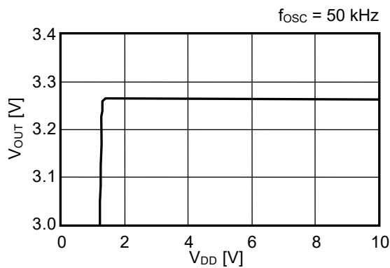
(4) Output Voltage (VOUT) vs. Power Supply Voltage (VDD) (V OUT = 3.3 V, V IN = 1.98 V, I OUT = 13.2 mA, V DD Separate Type)
