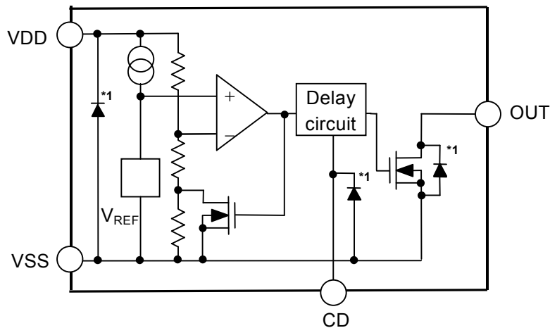
*1. Parasitic diode
