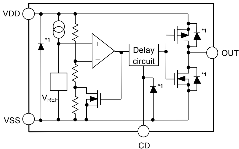
*1. Parasitic diode
