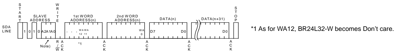
Figure 38. Page write cycle (BR24L32/64-W)
