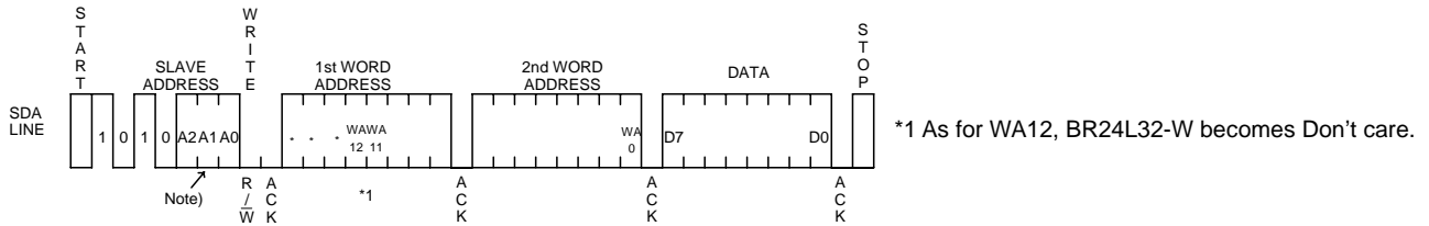
Figure 36. Byte write cycle (BR24L32/64-W)
