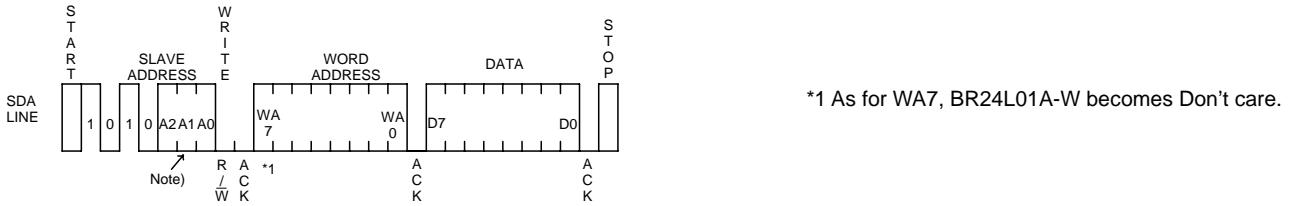
Figure 35. Byte write cycle (BR24L01A/02/04/08/16-W)
