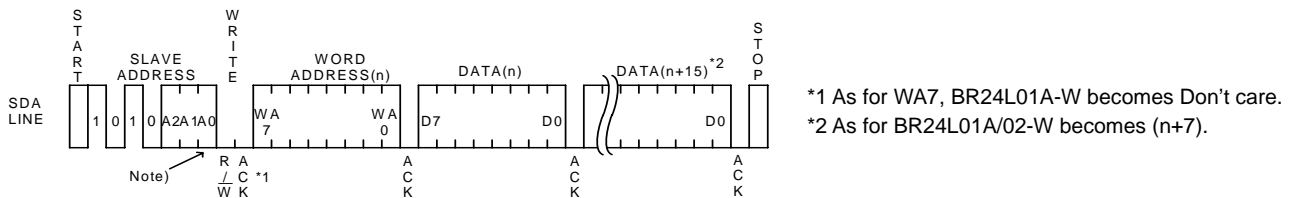
Figure 37. Page write cycle (BR24L01A/02/04/08/16-W)
