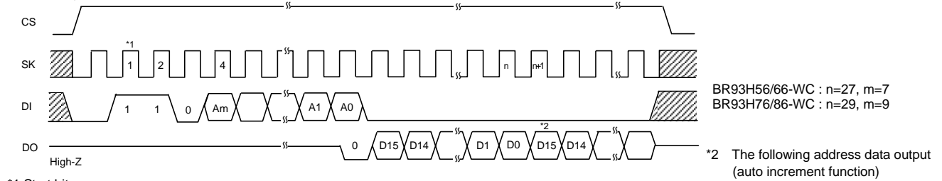
Figure 28. Read cycle
