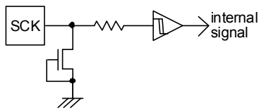
Figure 49. SCK input equivalent circuit
