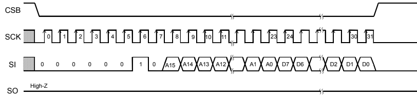
Figure 35. Write command
