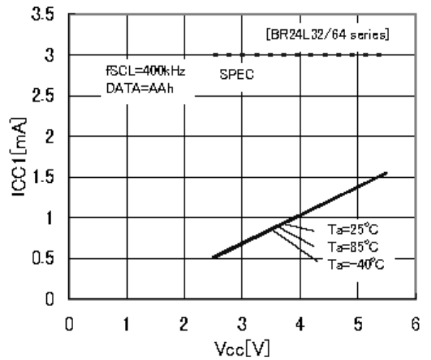
Figure 9. Current consumption at WRITE action ICC1 (fsc1=400kHz)
