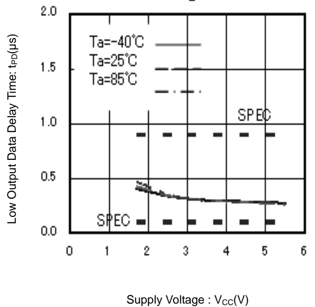
Figure 21. Low Output Data Delay Time vs Supply Voltage
