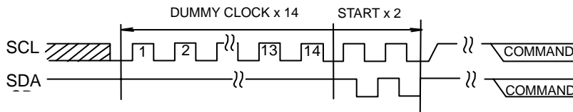
Figure 41-(a). DUMMY CLOCK x 14 + START + START
