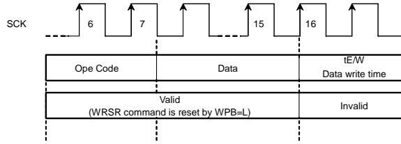
Figure 37. \overline{\text{WP}} valid timing (At inputting WRSR command)
