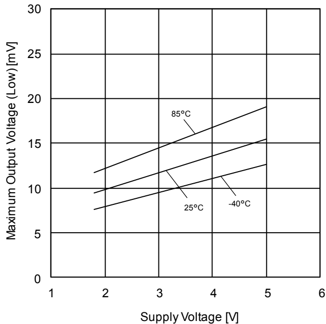
Figure 56. Maximum Output Voltage Low vs Supply Voltage ( R_L=2k\Omega )
