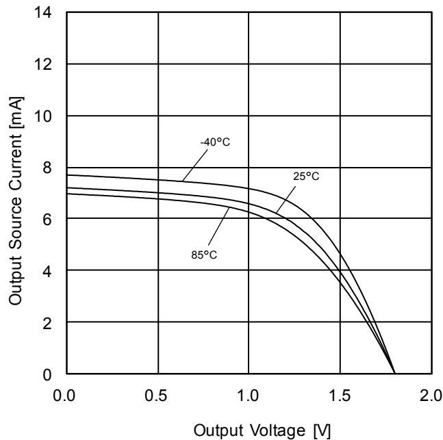
Figure 58. Output Source Current vs Output Voltage ( V_{DD}=1.8V )
