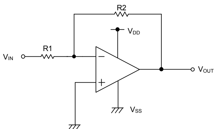
Figure 80. Inverting Amplifier Circuit
