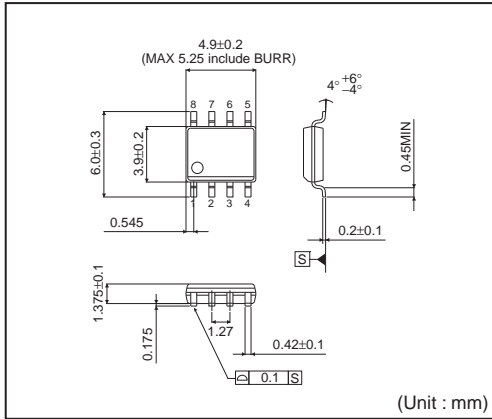
SOP8(TOP VIEW)
