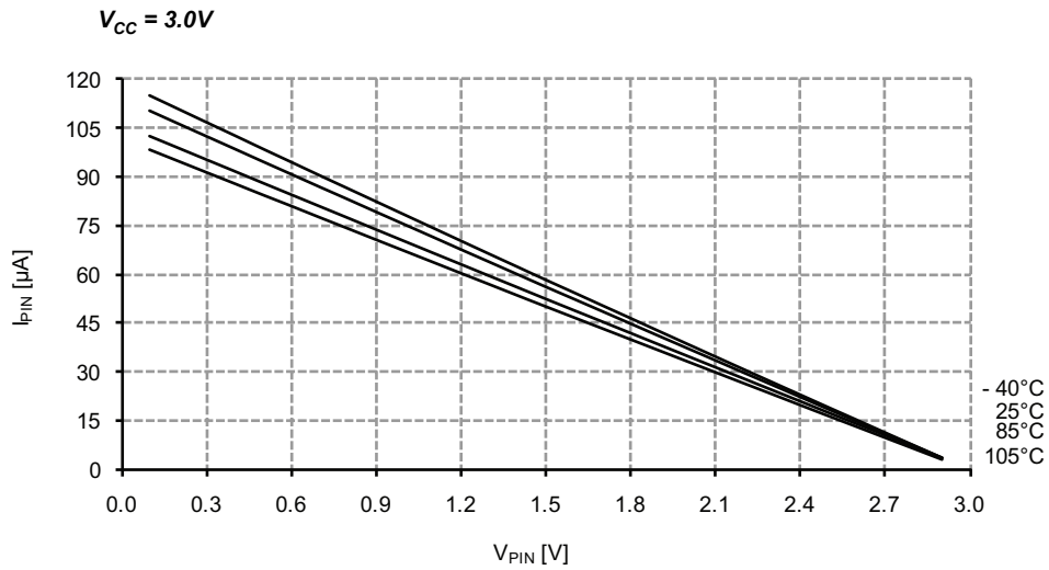
Figure 33-180. I/O Pin Pull-up Resistor Current vs. Input Voltage
