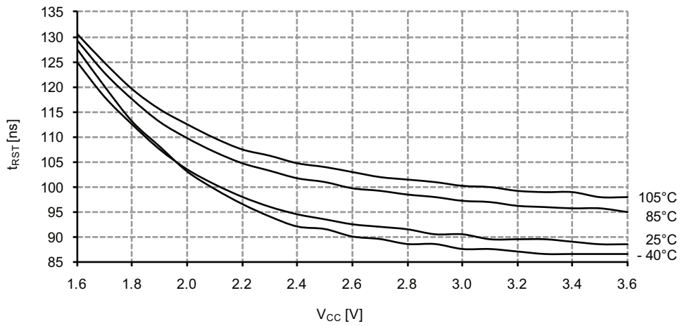
Figure 33-220. Minimum Reset Pin Pulse Width vs. V CC
