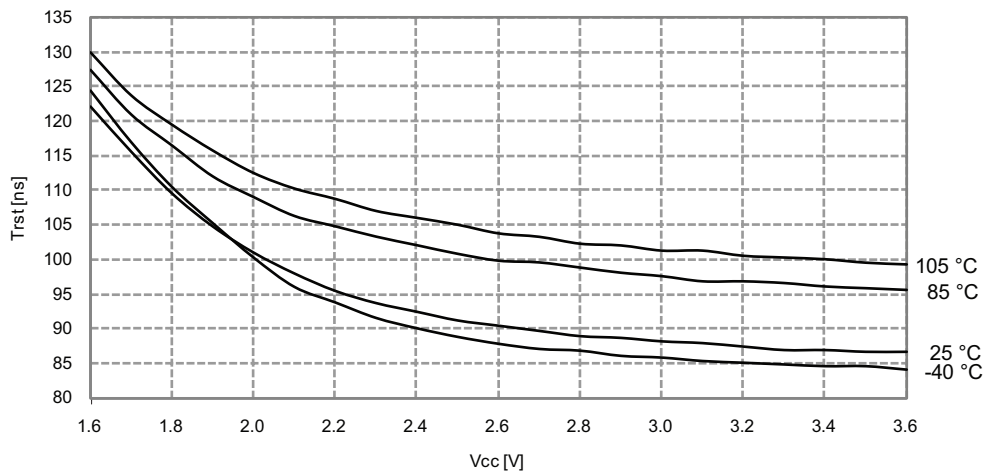
Figure 33-304. Minimum Reset Pin Pulse Width vs. V CC
