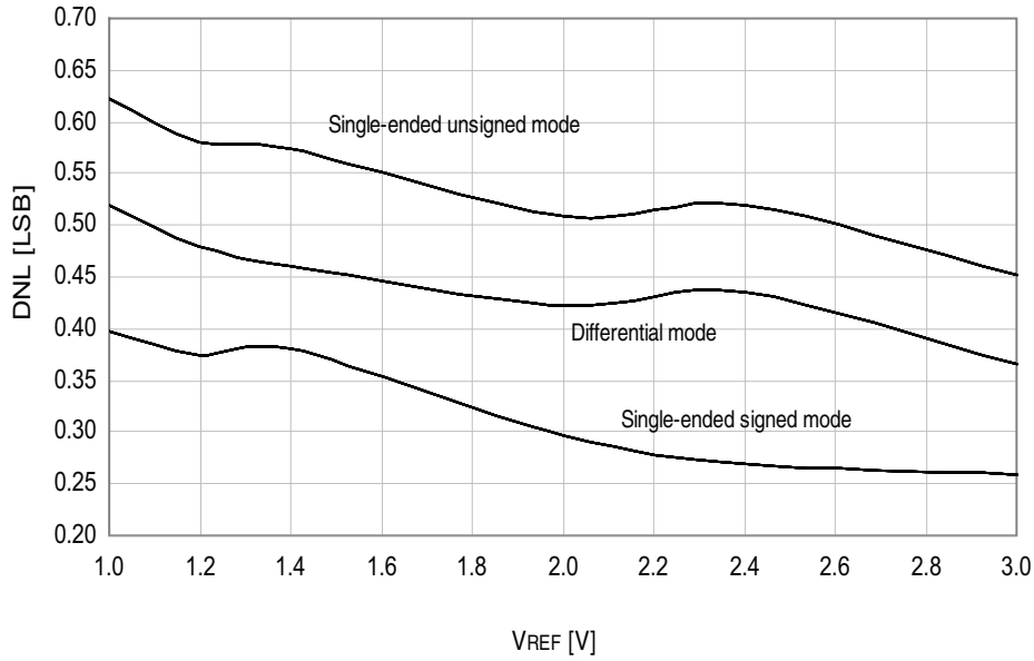
Figure 33-39. DNL Error vs. External V_{REF}
