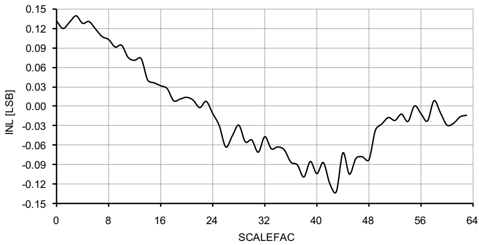
Figure 33-216. Voltage Scaler INL vs. SCALEFAC
