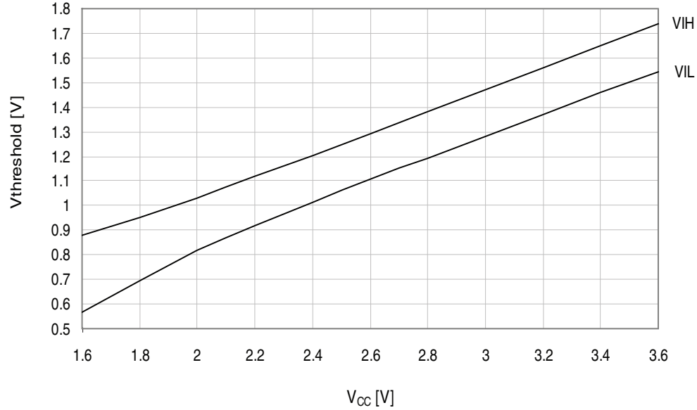
Figure 33-111. I/O Pin Input Threshold Voltage vs. V_{CC} T = 25^\circ\text{C}
