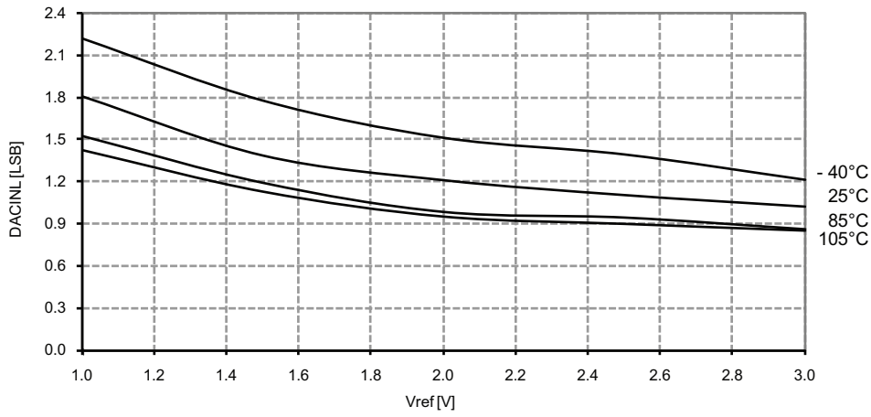
Figure 33-207. DAC INL Error vs. V_{REF} V_{CC} = 3.6V
