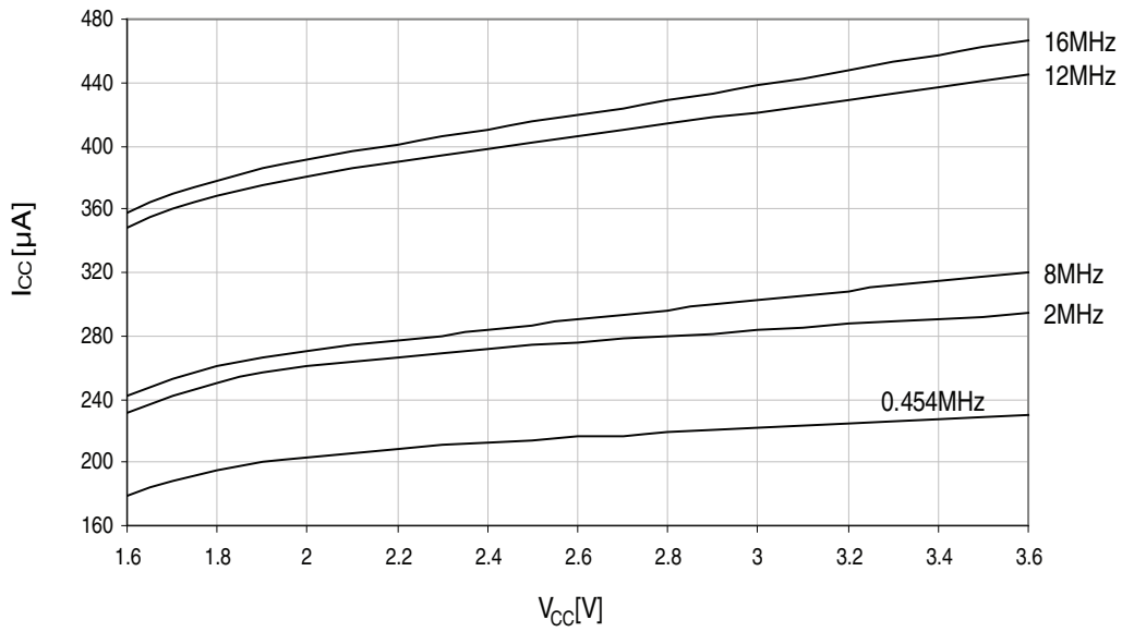
Figure 33-262. Standby Supply Current vs. V_{CC} T = 25^{\circ}C , running from different crystal oscillators
