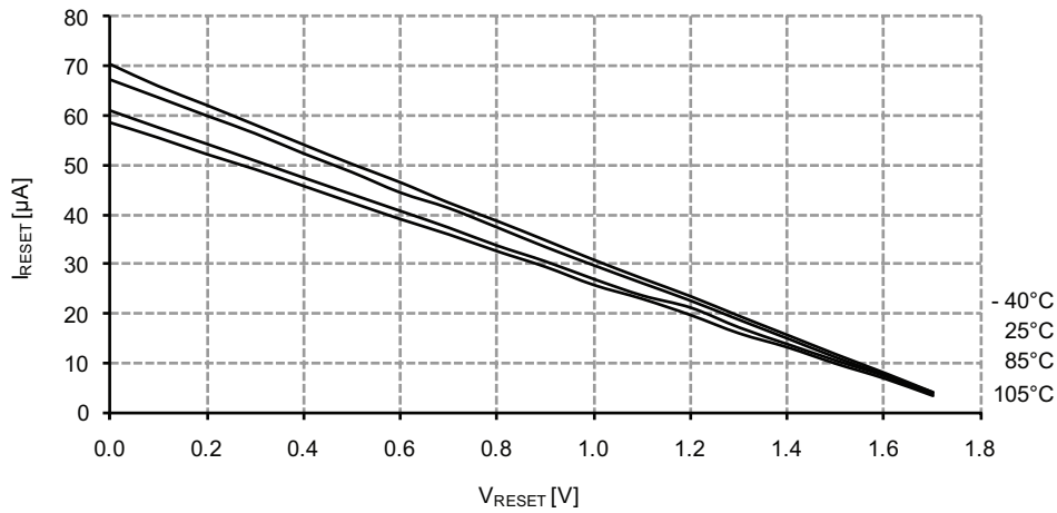
Figure 33-221. Reset Pin Pull-up Resistor Current vs. Reset Pin Voltage
