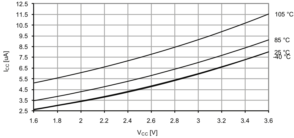
Figure 33-177. Standby Supply Current vs. V_{CC} Standby, f_{SYS} = 1MHz
