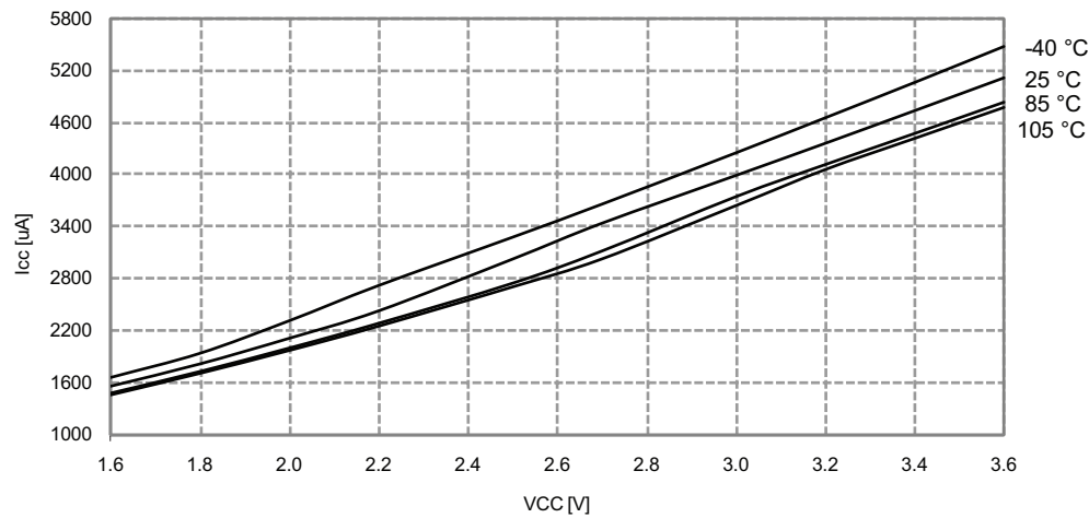
Figure 33-248. Active Mode Supply Current vs. V_{CC}
