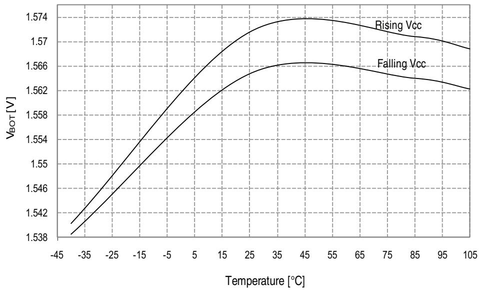
Figure 33-56. BOD Thresholds vs. Temperature
