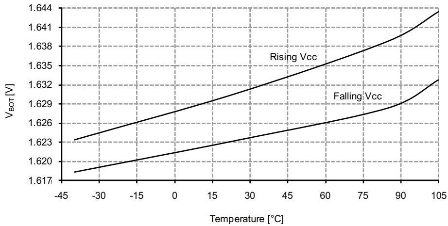
Figure 33-218. BOD Thresholds vs. Temperature
