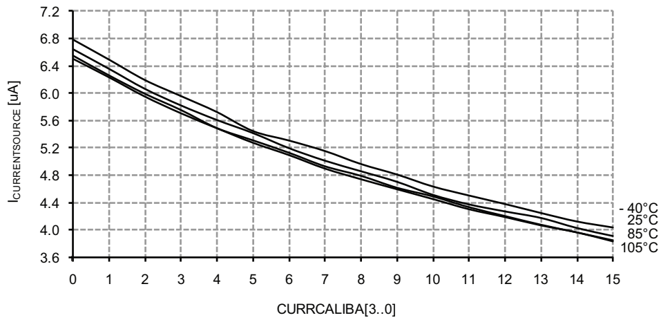
Figure 33-215. Analog Comparator Current Source vs. Calibration Value
