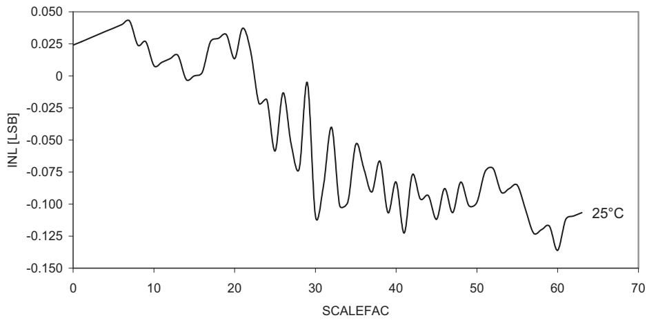
Figure 33-300. Voltage Scaler INL vs. SCALEFAC
