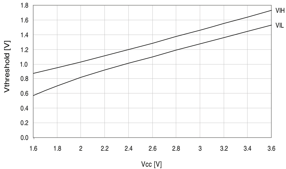
Figure 33-274. I/O Pin Input Threshold Voltage vs. V_{CC} T = 25^{\circ}\text{C}
