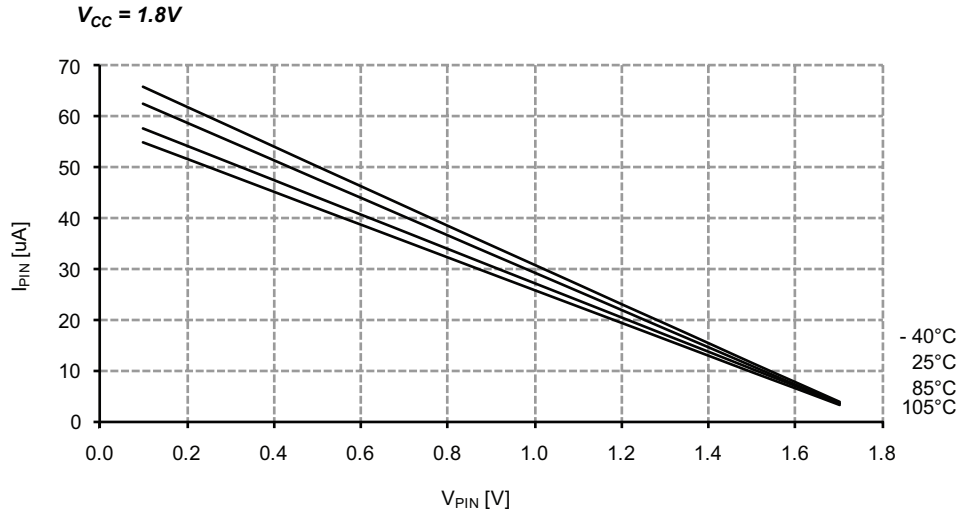
Figure 33-179. I/O Pin Pull-up Resistor Current vs. Input Voltage
