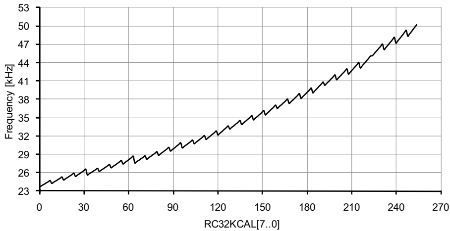
Figure 33-230. 32.768kHz Internal Oscillator Frequency vs. Calibration Value
