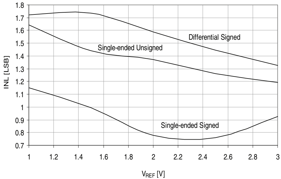
Figure 33-278. INL Error vs. External V_{REF}
