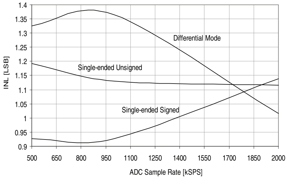
Figure 33-279. INL Error vs. Sample rate T = 25°C, V CC = 3.6V, V REF = 3.0V external
