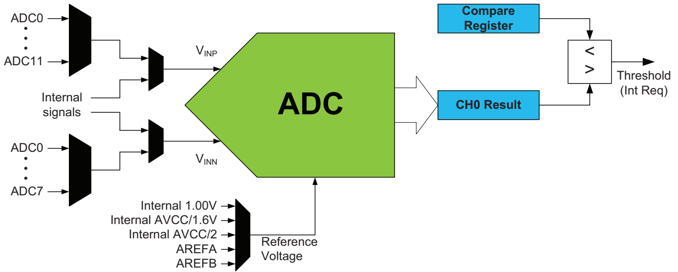
Figure 25-1. ADC overview
