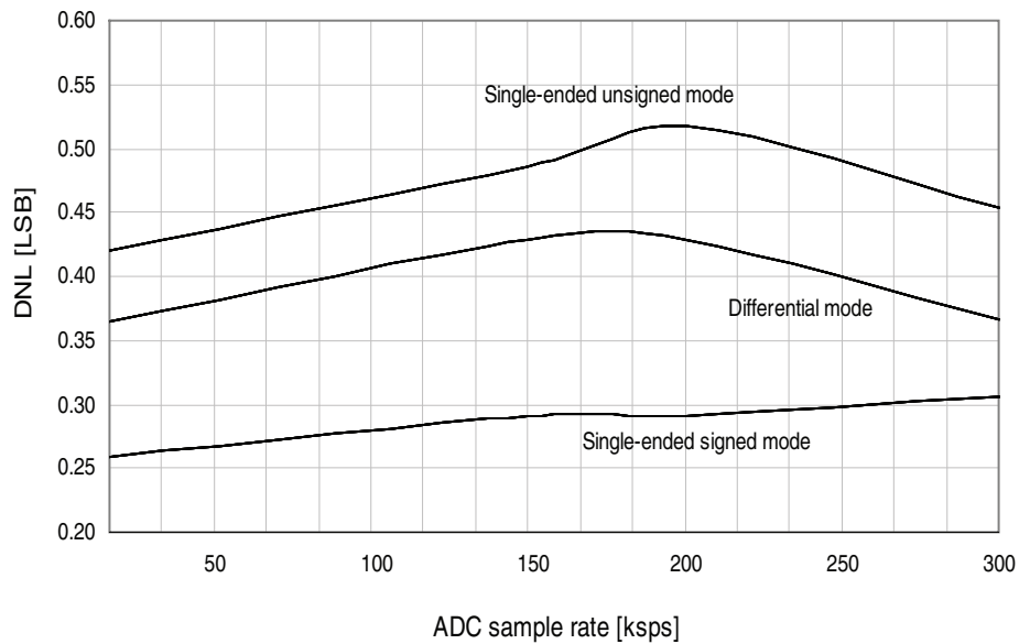
Figure 33-40. DNL Error vs. Sample Rate
