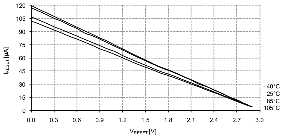
Figure 33-222. Reset Pin Pull-up Resistor Current vs. Reset Pin Voltage
