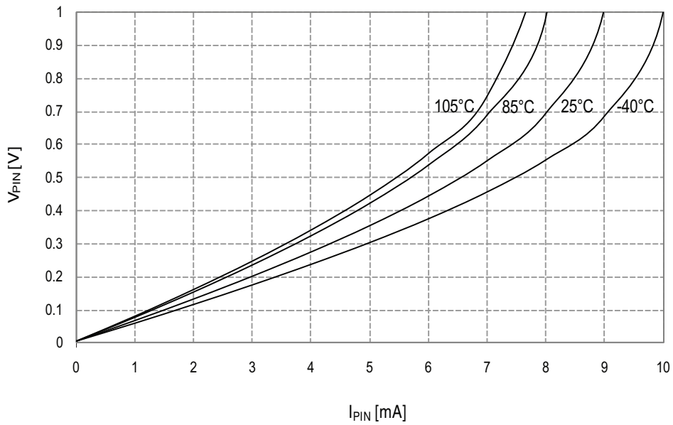
Figure 33-28. I/O Pin Output Voltage vs. Sink Current V_{CC} = 1.8V
