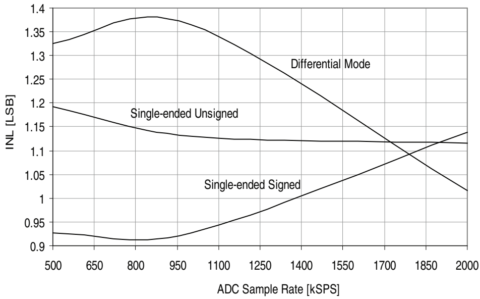
Figure 33-279. INL Error vs. Sample rate T = 25^{\circ}\text{C} , V_{CC} = 3.6\text{V} , V_{REF} = 3.0\text{V external}
