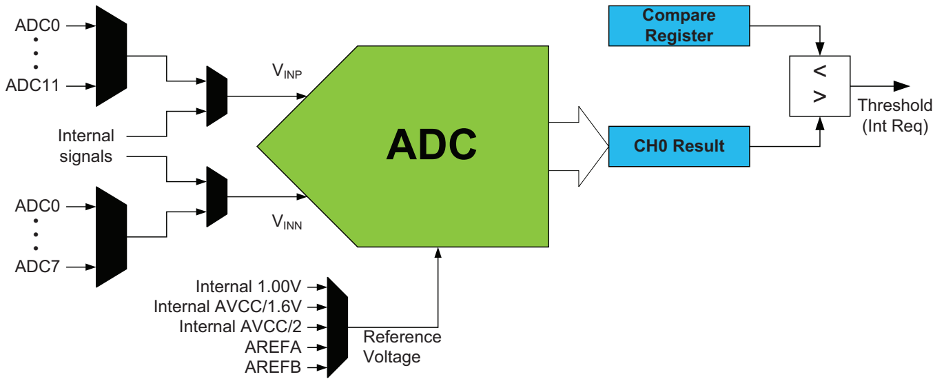
Figure 25-1. ADC overview
