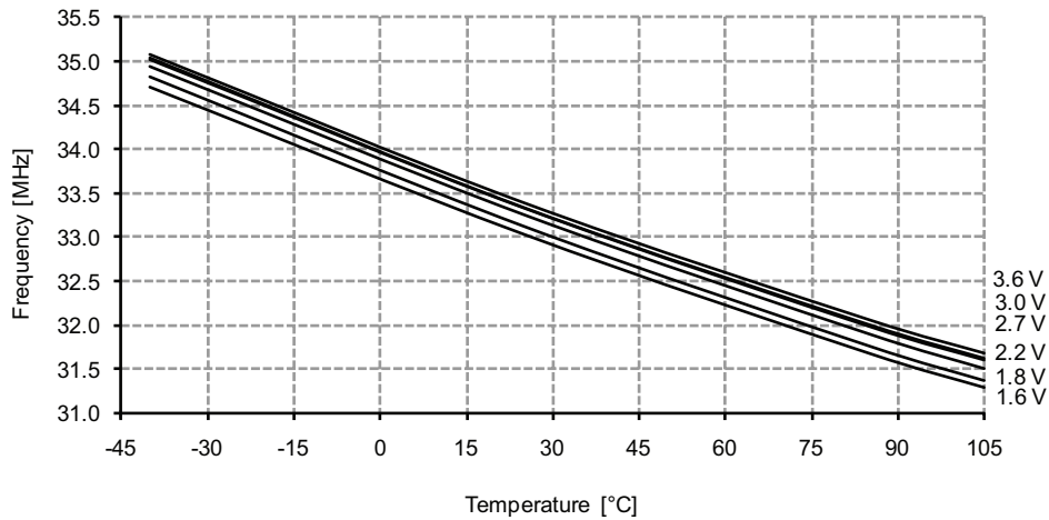
Figure 33-234. 32MHz Internal Oscillator Frequency vs. Temperature
