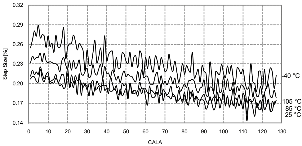
Figure 33-320. 32MHz Internal Oscillator CALA Calibration Step Size V_{CC} = 3.0V
