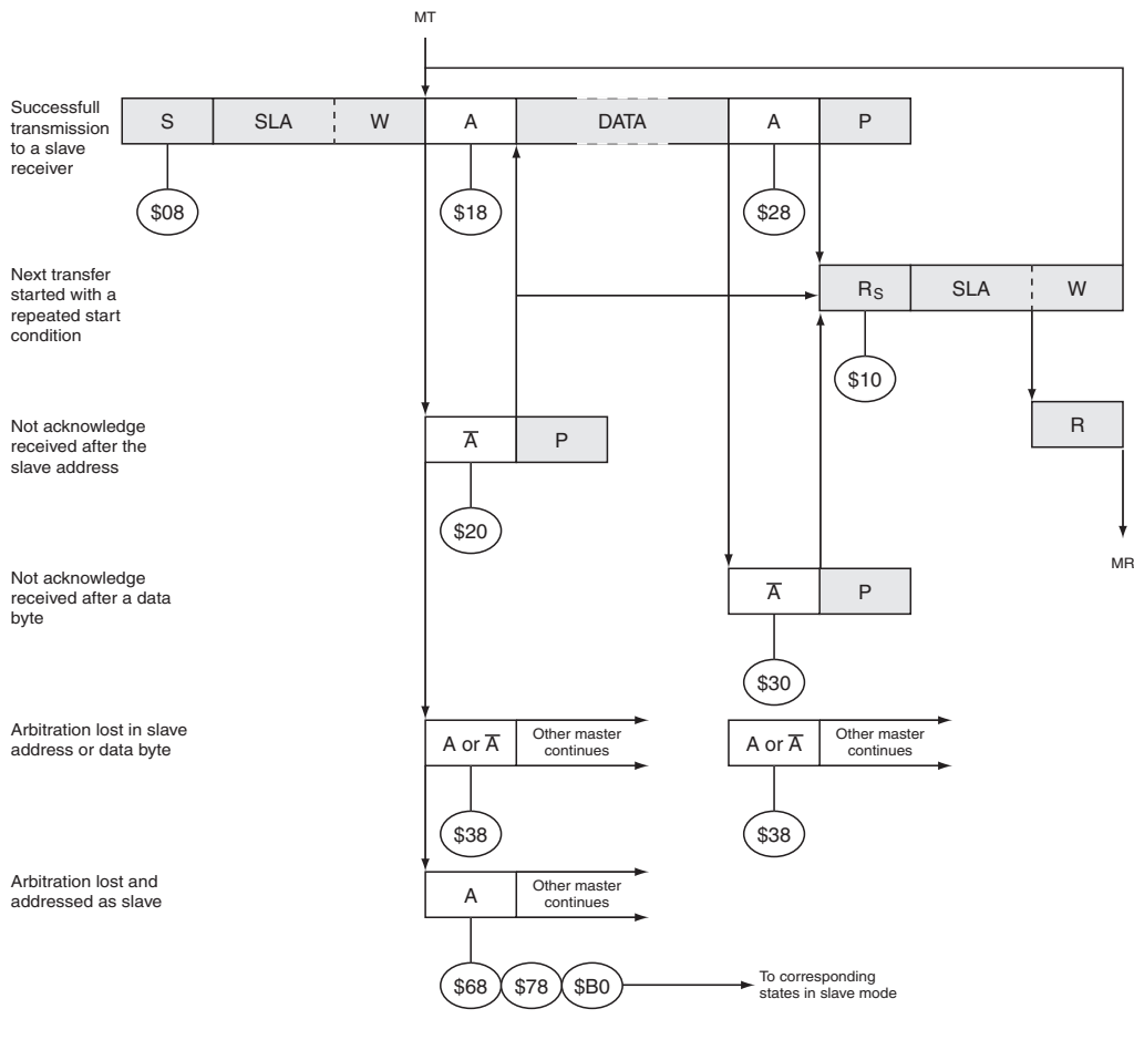
Figure 22-12. Formats and States in the Master Transmitter Mode
