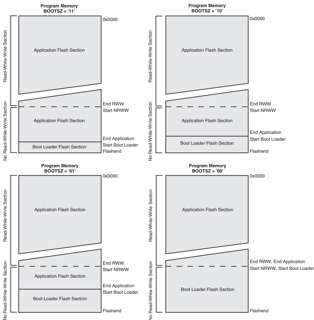
Figure 27-2. Memory Sections
