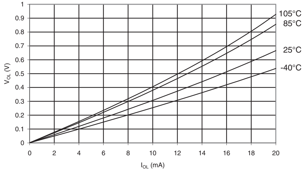
Figure 31-258. ATmega168PA: I/O Pin Output Voltage vs. Sink Current ( V_{CC} = 5V )
