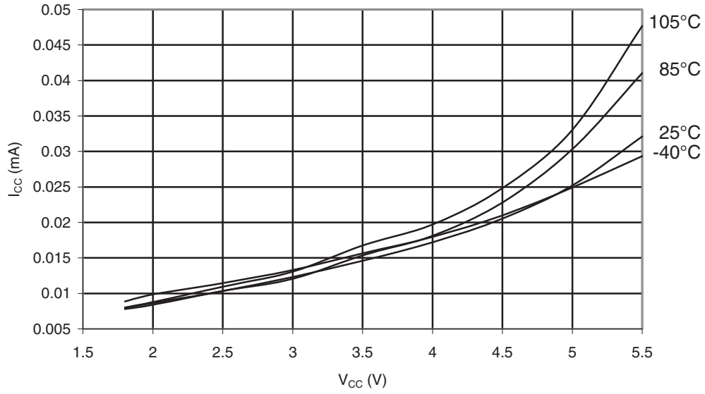
Figure 31-340. ATmega328P: Idle Supply Current vs. V_{CC} (Internal RC Oscillator, 1MHz)
