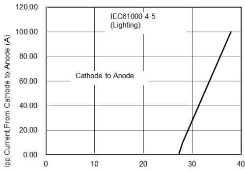
Figure 5 Clamping Voltage Characteristic
