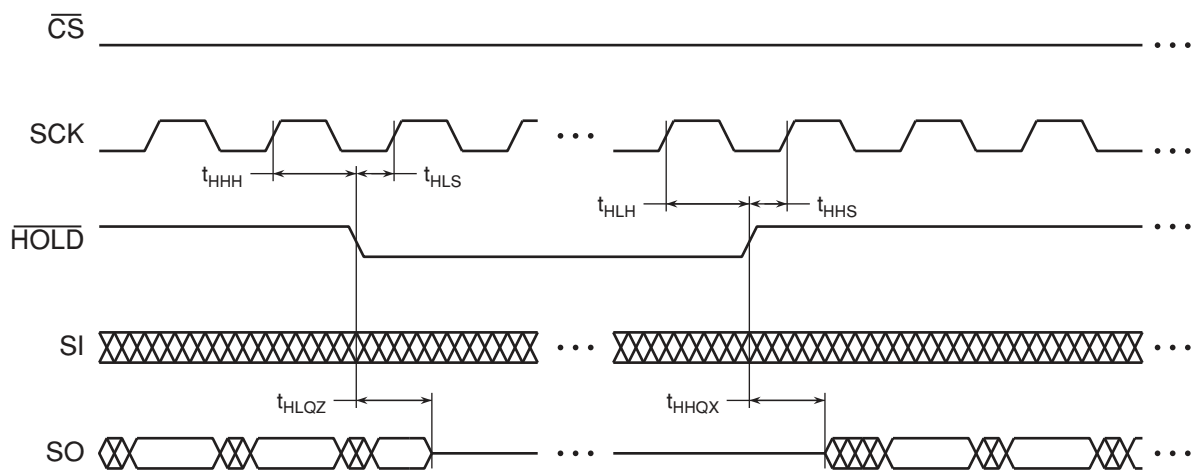
Figure 8-16. \overline{HOLD} Timing – Serial Output
