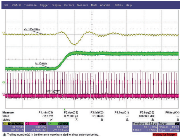
Fig. 28 - Load Step, 12 A to 24 A, 1 A/ \mu\text{s} , t = 10\text{ }\mu\text{s}/\text{div}
