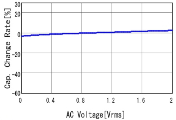
■RDER72A104K1M1H03A C-AC Voltage capchange, DC0V, 25.0
