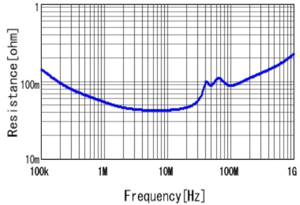
■RDER72A104K1M1H03A R DC0V, 25degC
