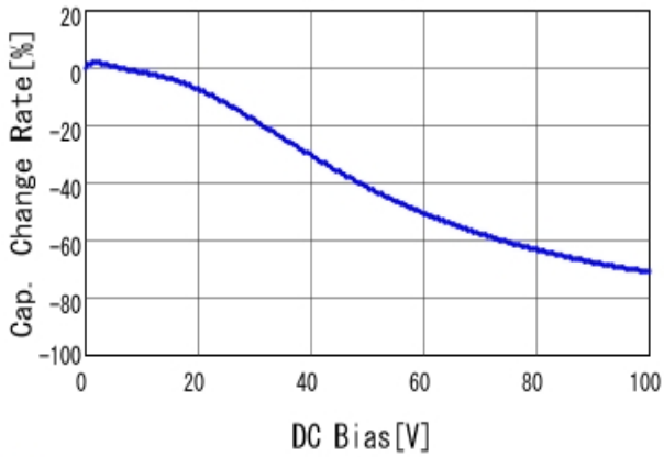
■RDER72A104K1M1H03A C-DC bias capchange, 25.0degC, AC1
