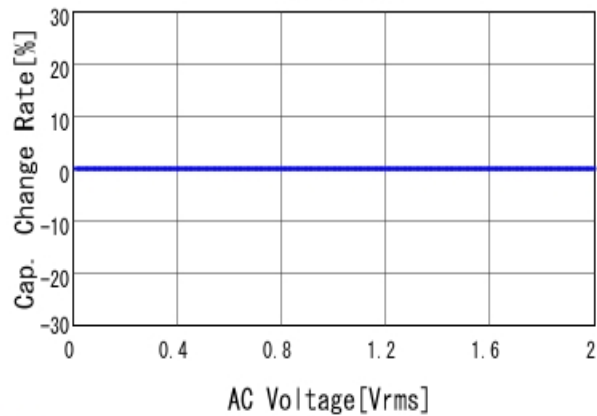
■ GRM1885C1HR60BA01 C-AC Voltage capchange, DC0V, 25.0d
