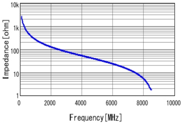
■ GRM1885C1HR60BA01 |Z| DC0V, 25degC
