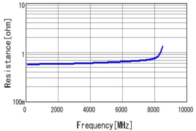
■ GRM1885C1HR60BA01 R DC0V, 25degC
