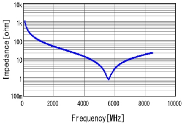
■ GRM1885C1H1R5WA01 |Z| DCOV, 25degC
