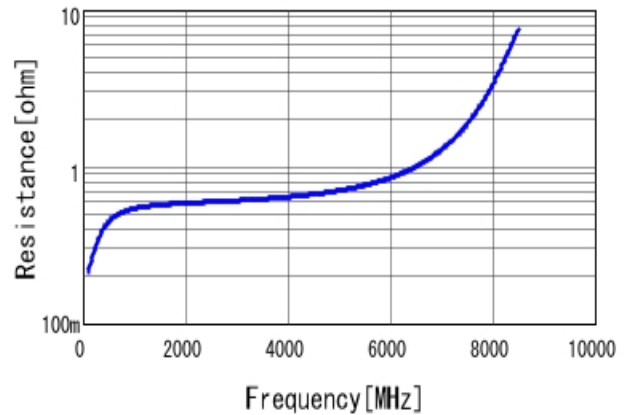
■ GRM1885C1H1R5WA01 R DCOV, 25degC
