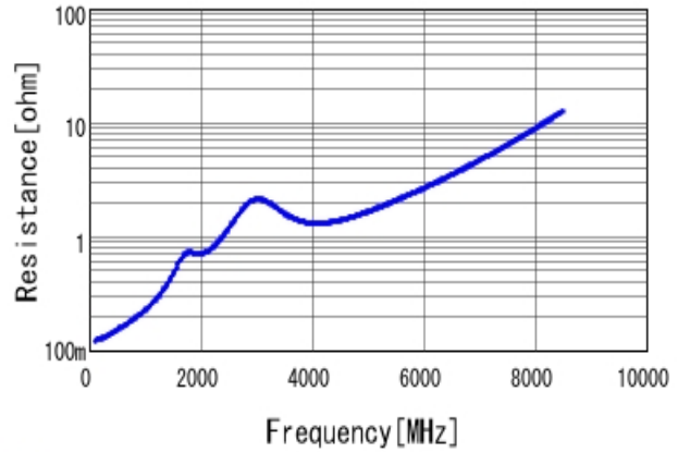
■ GRM1885C1H101GA01 R DCOV, 25degC
