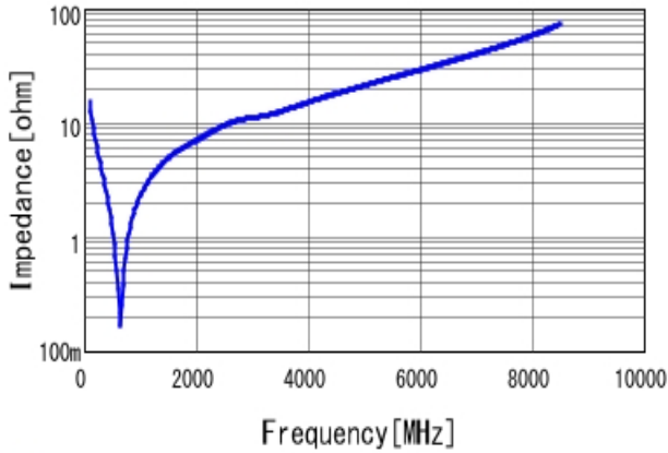
■ GRM1885C1H101GA01 |Z| DCOV, 25degC
