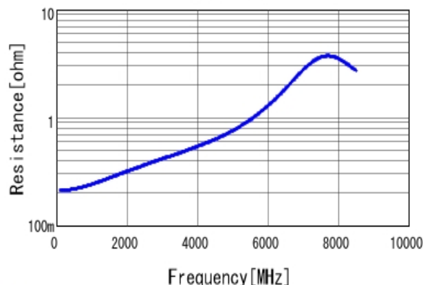
■ GRM1555C1H6R0WA01 R DCOV, 25degC
