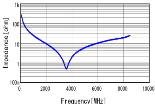
■ GRM1555C1H6R0WA01 |Z| DCOV, 25degC
