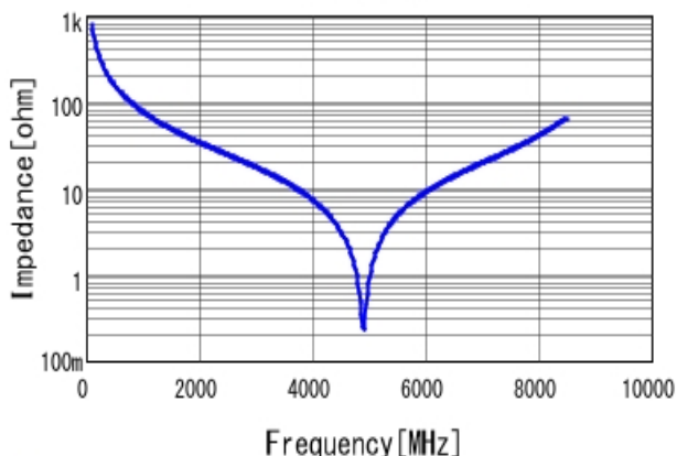
■ GQM1885C2A2R0CB01 |Z| DCOV, 25degC
