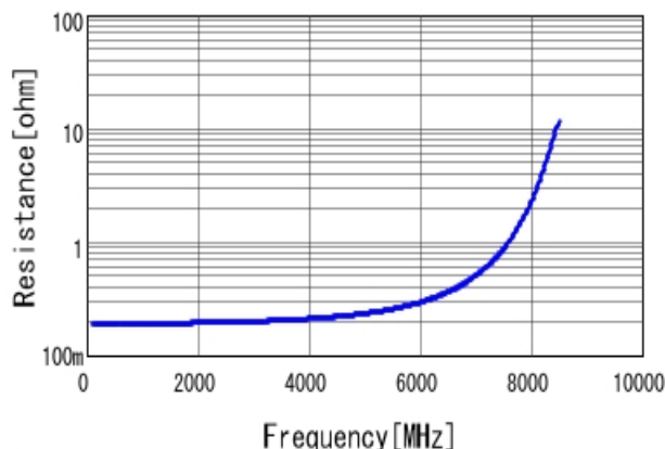
■ GQM1885C2A2R0CB01 R DCOV, 25degC
