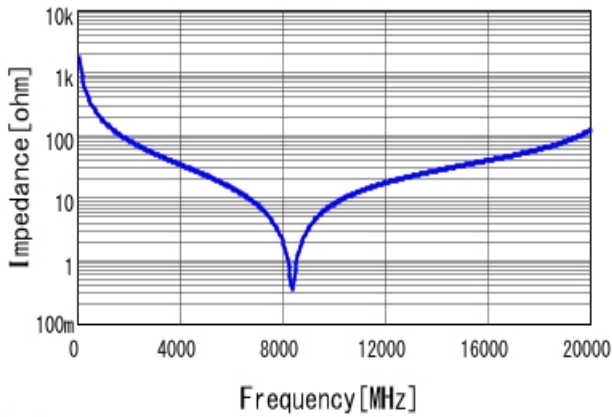
■GJM1555C1HR90BB01 |Z| DC0V, 25degC
