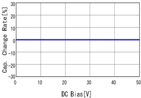
■GJM1555C1HR90BB01 C-DC bias capchange, 25.0degC, AC1V
