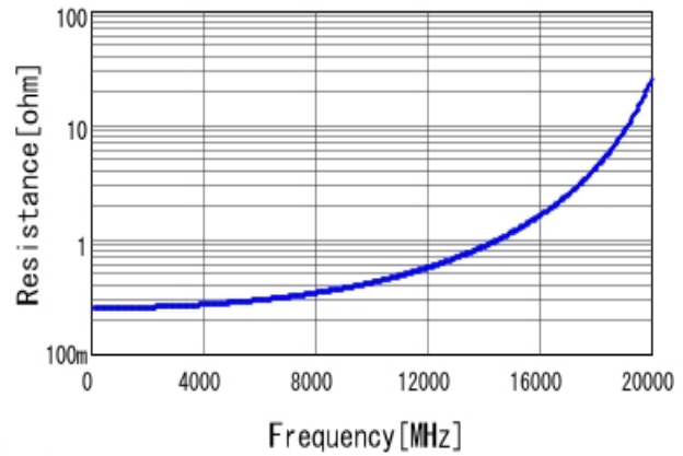
■GJM1555C1HR90BB01 R DC0V, 25degC
