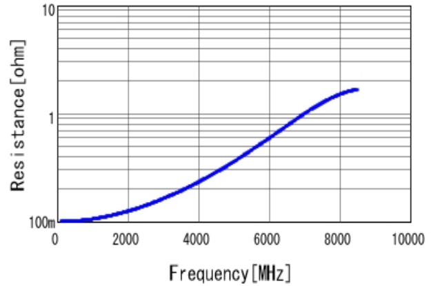
■GJM1555C1H6R0WB01 R DC0V, 25degC
