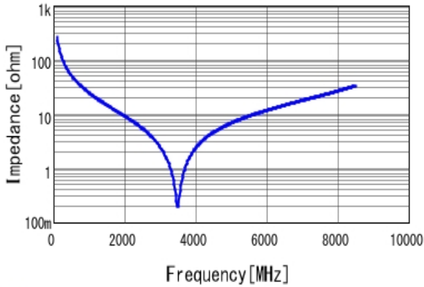
■GJM1555C1H6R0WB01 |Z| DC0V, 25degC
