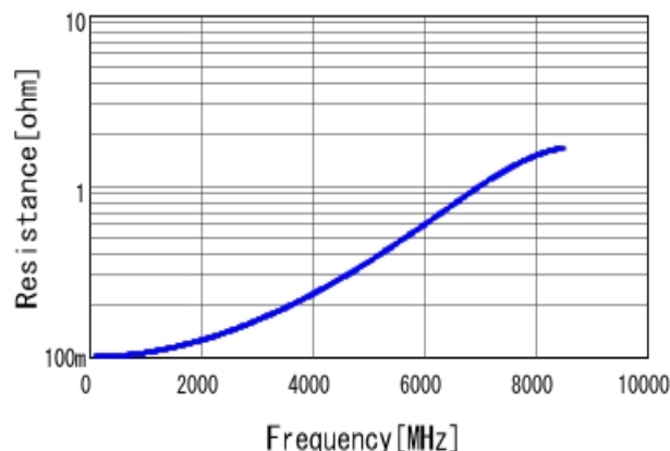
■ GJM1555C1H6R0BB01 R DC0V, 25degC
