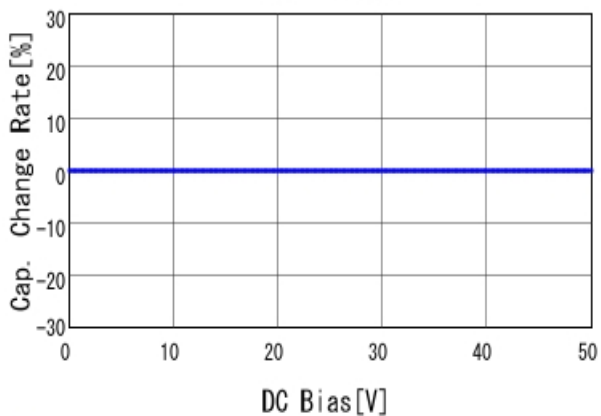
■ GJM1555C1H6R0BB01 C-DC bias capchange, 25.0degC, AC1V
