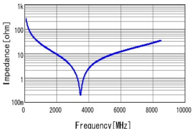
■ GJM1555C1H6R0BB01 |Z| DC0V, 25degC
