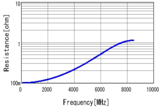
■GJM1555C1H5R1CB01 R DC0V, 25degC
