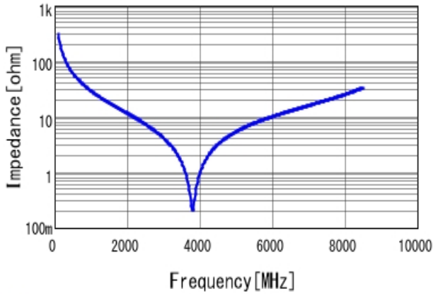
■GJM1555C1H5R1CB01 |Z| DC0V, 25degC
