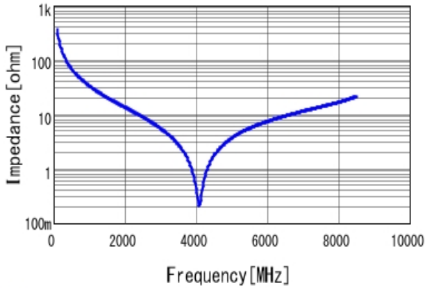
■ GJM1555C1H4R5BB01 |Z| DC0V, 25degC
