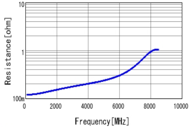
■ GJM1555C1H4R5BB01 R DC0V, 25degC
