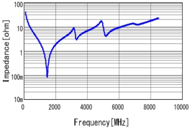
■GJM1555C1H390FB01 |Z| DC0V, 25degC
