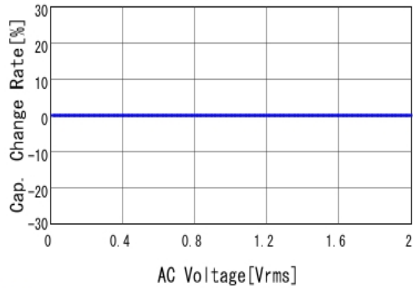
■GJM1555C1H390FB01 C-AC Voltage capchange, DC0V, 25.0d
