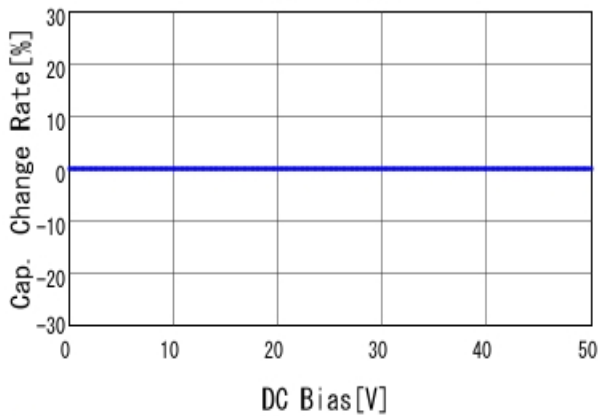
■GJM1555C1H200GB01 C-DC bias capchange, 25.0degC, AC1V
