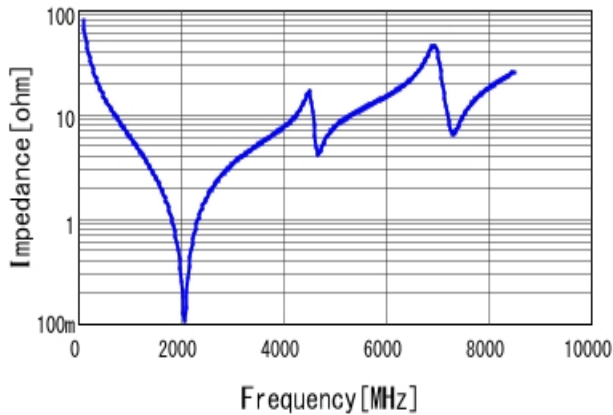
■GJM1555C1H200GB01 |Z| DC0V, 25degC
