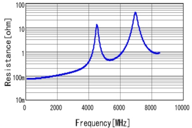
■GJM1555C1H200GB01 R DC0V, 25degC
