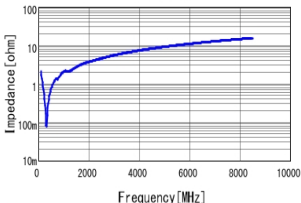
■ GCM1555C1H681FA16 |Z| DC0V, 25degC
