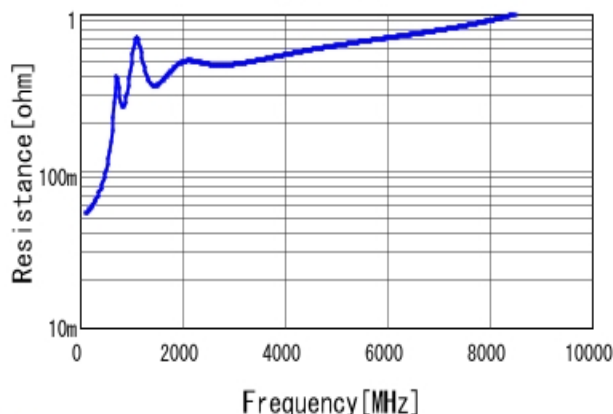
■ GCM1555C1H681FA16 R DC0V, 25degC
