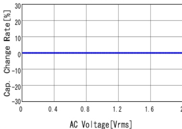
■ GCM1555C1H681FA16 C-AC Voltage capchange, DC0V, 25.0d
