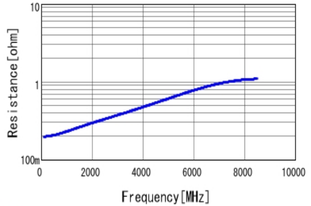
GCM0335C1E100JA16 R DC0V, 25degC
