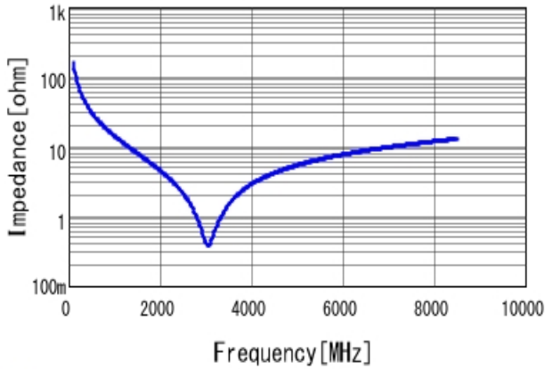
GCM0335C1E100JA16 |Z| DC0V, 25degC
