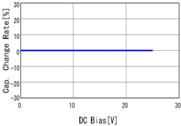
GCM0335C1E100JA16 C-DC bias capchange, 25.0degC, AC1V
