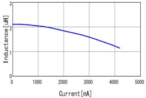
■ 1277AS-H-2R2M L-Current 20degC
