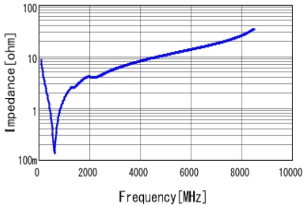
■ GCM1555C1H181JA16 |Z| DC0V, 25degC
