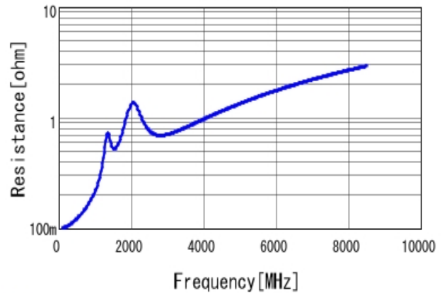
■ GCM1555C1H181JA16 R DC0V, 25degC
