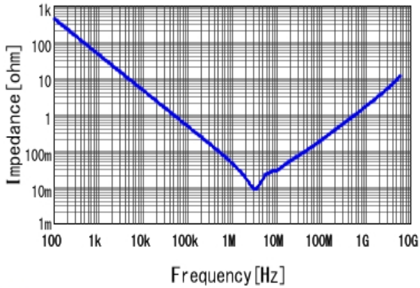
■GCJ188C70J475ME02 |Z| DC0V, 25degC
