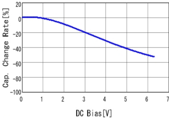
■GCJ188C70J475ME02 C-DC bias capchange, 25.0degC, AC1V
