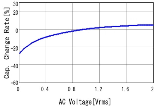
■GCJ188C70J475ME02 C-AC Voltage capchange, DC0V, 25.0d
