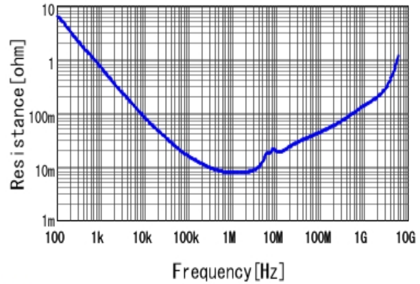
■GCJ188C70J475ME02 R DC0V, 25degC
