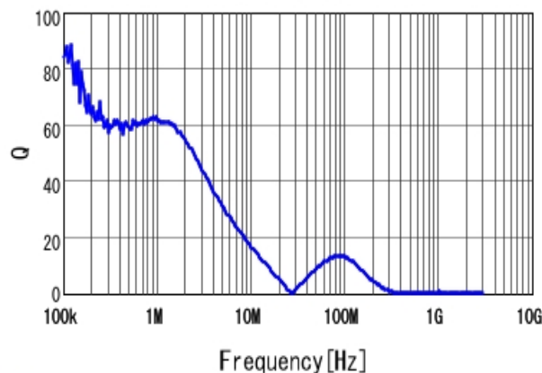
■ FDVE0630-H-3R3M Q
