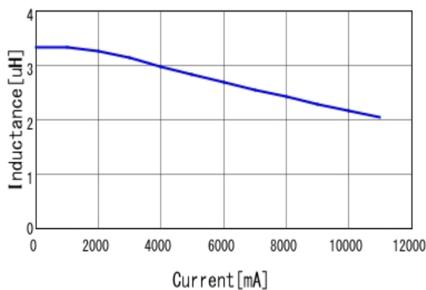
■ FDVE0630-H-3R3M L-Current 20degC
