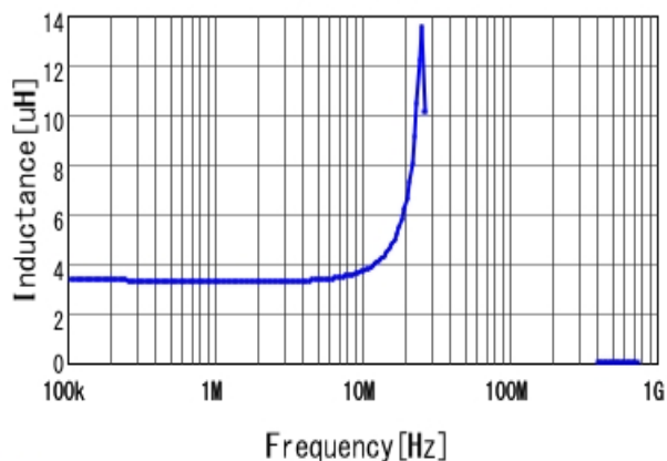
■ FDVE0630-H-3R3M L
