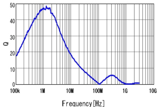
■ FDSD0420-H-R47M Q
