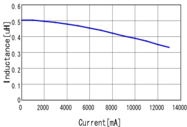
■ FDSD0420-H-R47M L-Current 20degC
