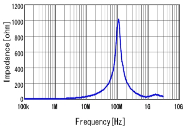
■ FDSD0420-H-R47M |Z|
