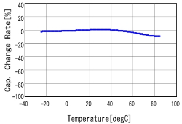
■DE1B3RA681KA4BN01F C-Temp. capchange, DCOV, AC1Vrms
