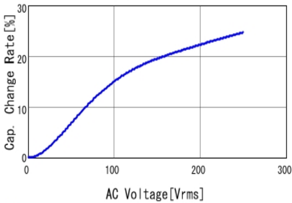
■DE1B3RA681KA4BN01F C-AC Voltage capchange, DCOV, 20.0
