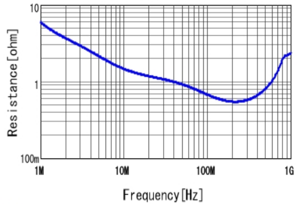
■DE1B3RA681KA4BN01F R DCOV, 20degC
