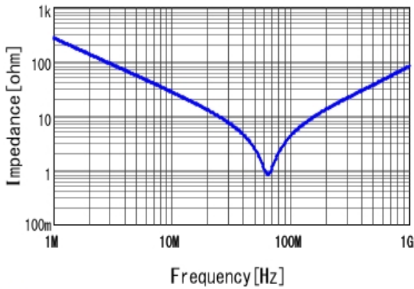
■DE1B3RA681KA4BN01F |Z| DCOV, 20degC
