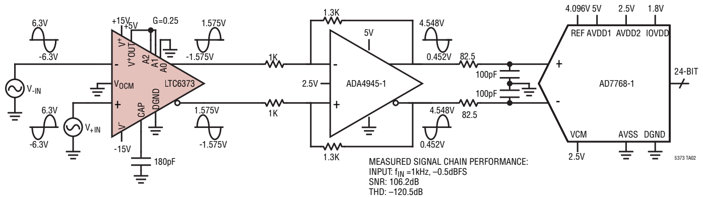
LTC6373 Driving the AD7768-1 \Sigma - \Delta ADC through a Fully Differential ADC Driver (ADA4945-1)
