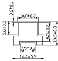
TUBE MECHANICAL DIMENSION
