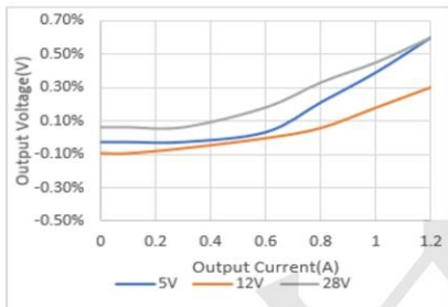
Load Regulation
