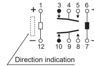
Schematic 2 coil latching (Bottom view)
