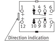
Schematic 2 coil latching (Bottom view)
