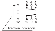
Schematic (Bottom view) Single side stable
