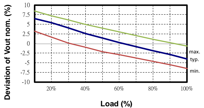
5VDC Output
