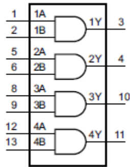
Figure 1. Functional diagram
