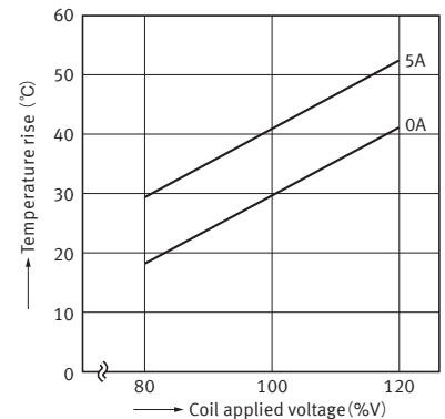
3.-(3) Coil temperature rise (2 Form A)
