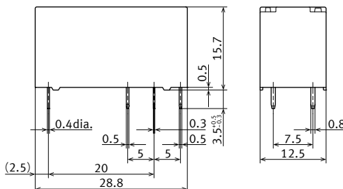
External dimensions
