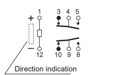
Schematic (Bottom view) Single side stable
