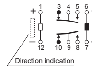
Schematic 2 coil latching (Bottom view)
